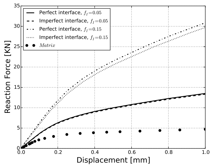
Figure 7: Reaction force versus displacement.
